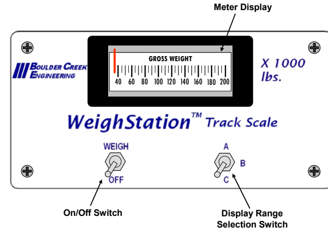
Figure 2: Faceplate Controls
